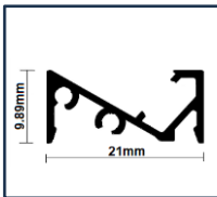
PERFIL SHELF-S
